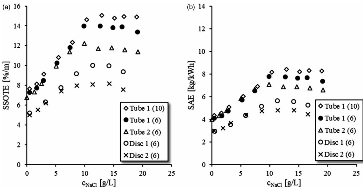
Figure 7 | Average SSOTE values as function of c_{NaCl} (a); average SAE values as a function of c_{NaCl} (b) calculated with isochoric power formula ( \eta = 0.60 ).
