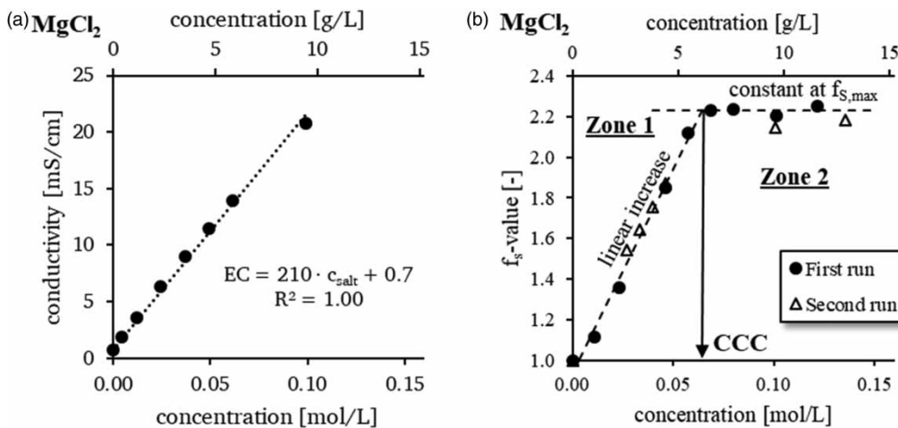
Figure 2 | Measuring CCC: calibration line for calculating \text{MgCl}_2 concentration by measuring conductivity (a); determining CCC of \text{MgCl}_2 by oxygen transfer test results in lab-scale experiments (b).
