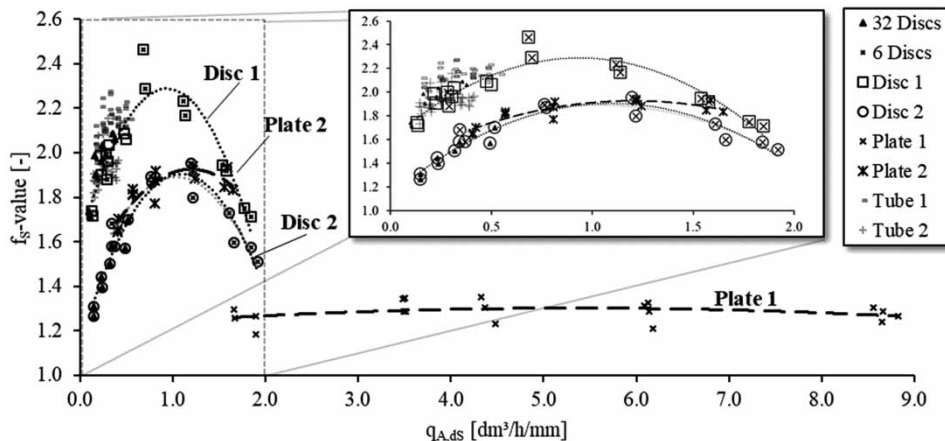
Figure 6 | f_S -value as a function of the airflow rate per slit and slit length ( q_{A,dS} ) for different diffuser types and c_{NaCl} > CCC_{NaCl} .
