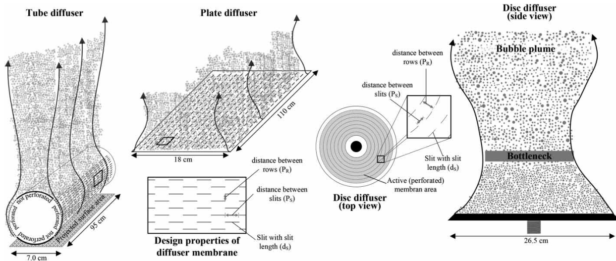
Figure 1 | Schematic representation of the tested diffuser types and the definition of parameters of membrane design.
