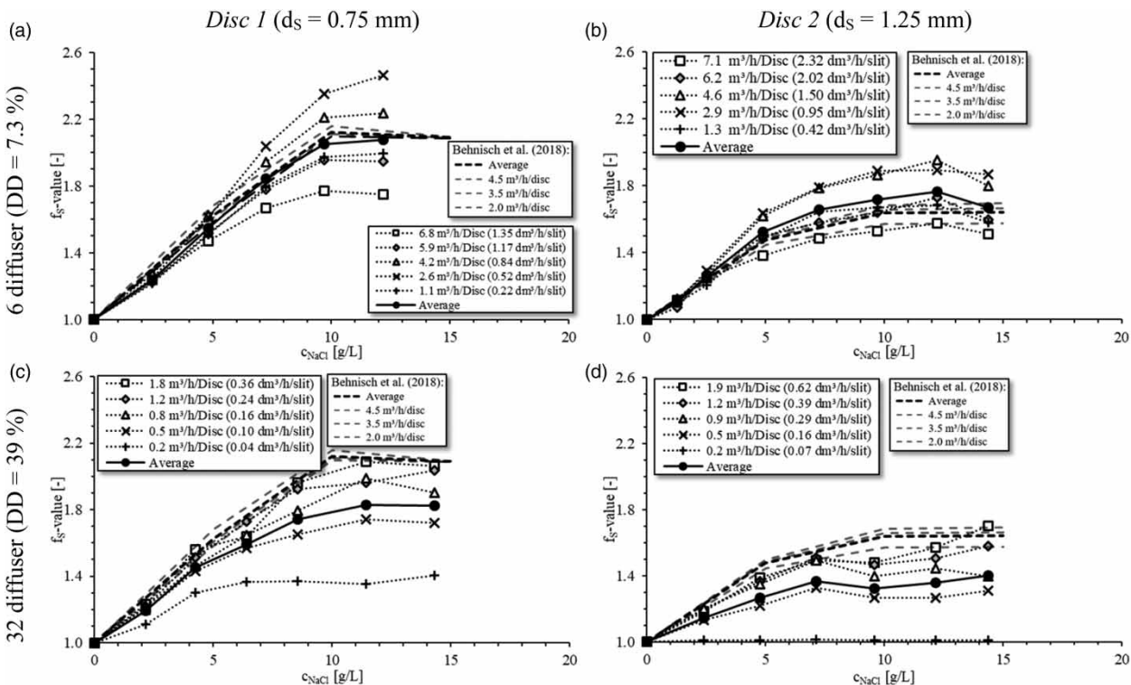
Figure 3 | f_S -values as function of c_{\text{NaCl}} from disc diffusers for different Q_{A,Disc} and Q_{A,Slit} supplemented by results of lab-scale experiments described in Part I of the present paper.
