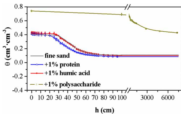
Figure 4 | Soil-water characteristic curves of fine sand with different media; \theta is the volumetric water content and h is the matric head.
