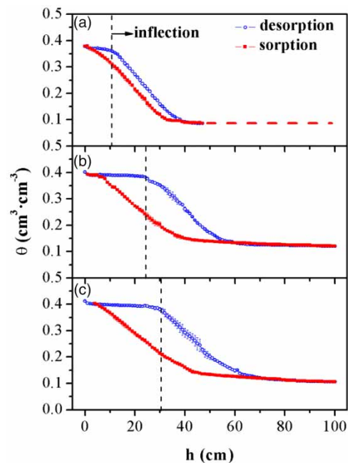
Figure 3 | Soil–water characteristic curves of sandy soils: (a) coarse sand, (b) medium sand, and (c) fine sand; \theta is the volumetric water content and h is the matric head.
