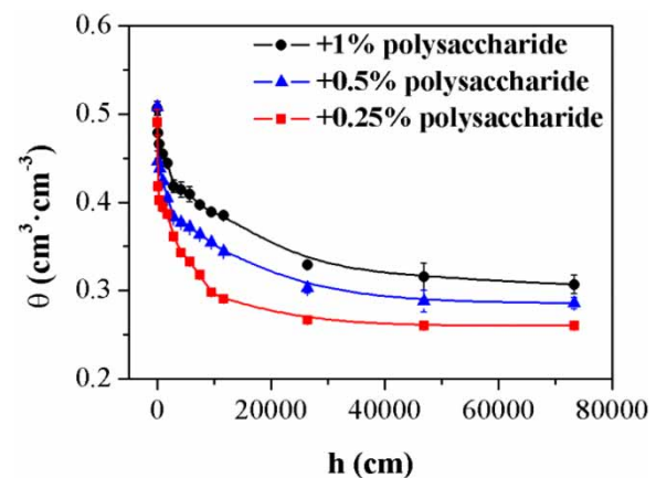
Figure 7 | Soil–water characteristic curves of fine sand with different polysaccharide concentrations; \theta is the volumetric water content and h is the matric head.
