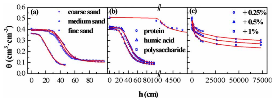
Figure 8 | Experimental SWCCs fitted using the van Genuchten model: (a) sandy soils of different sizes, (b) fine sands with different analogs added, (c) fine sands with different proportions of polysaccharides added.
