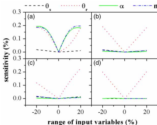
Figure 9 | Results of the sensitivity analysis of four media: (a) fine sandy soil, (b) sand +1% protein, (c) sand +1% humic acid, and (d) sand +1% polysaccharide mixture.
