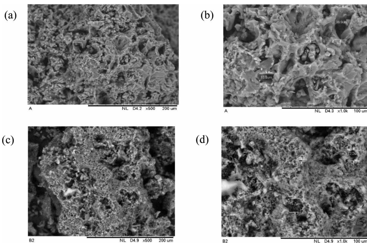
Figure 4 | SEM images of ((a) and (b)) SA and ((c) and (d)) SB at ×500 ((a) and (c)) and ×1,000 ((b) and (d)) magnifications.
