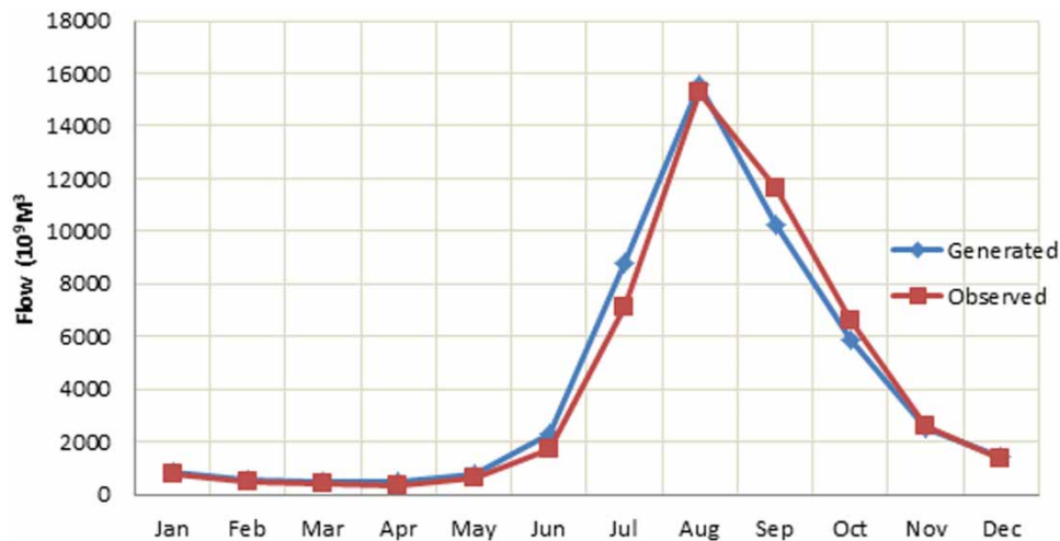
Figure 3 | Mean monthly hydrographs of observed and generated flow ( 10^9 m 3 ).
