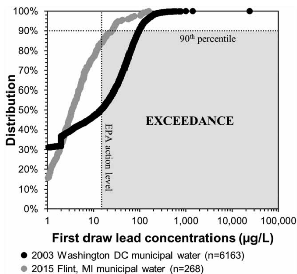
Figure 1 | Representative histogram of WLLs during the Flint and Washington DC lead in water crises (Edwards et al. 2009; Pieper et al. 2018a).
