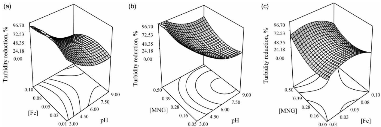
Figure 6 | 3-D response surface plots of (a) pH and concentration of Fe, (b) pH and concentration of MNG, and (c) concentration of Fe and MNG.
