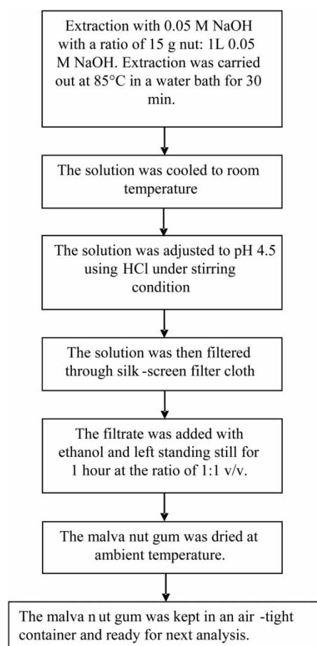
Figure 1 | Schematic diagram of MNG extraction process.
