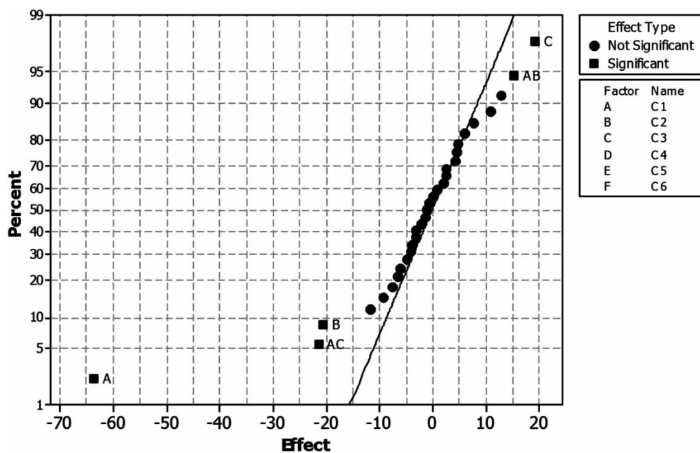
Figure 5 | Normal probability plot of the effects of MNG in single mixing mode. A: pH, B: Concentration of Fe, C: Concentration of MNG, D: Mixing speed, E: Mixing time, F: sedimentation time.
