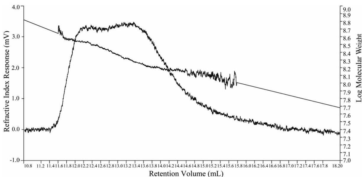
Figure 2 | Elution chromatography (refractive index signal) of MNG analysed by GPC.
