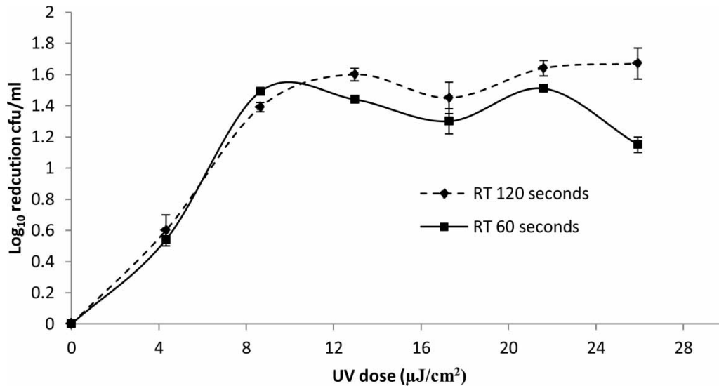
Figure 3 | Log 10 reduction of Bacillus cereus endospores via a flow through pulsed UV system at an RT of 120 seconds and a flow rate of 24 L/h, and at a 60-second RT and a flow rate of 30 L/h (±SD).
