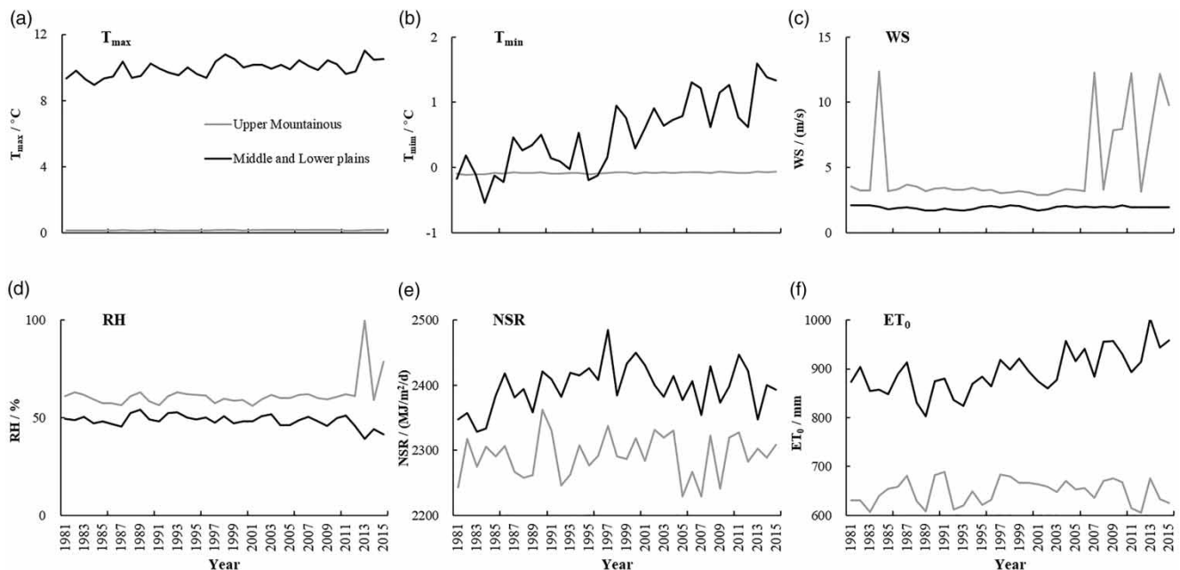
Figure 2 | Variations of five climatic factors and ET_0 from 1981 to 2015 in the two regions of the SYRB.
