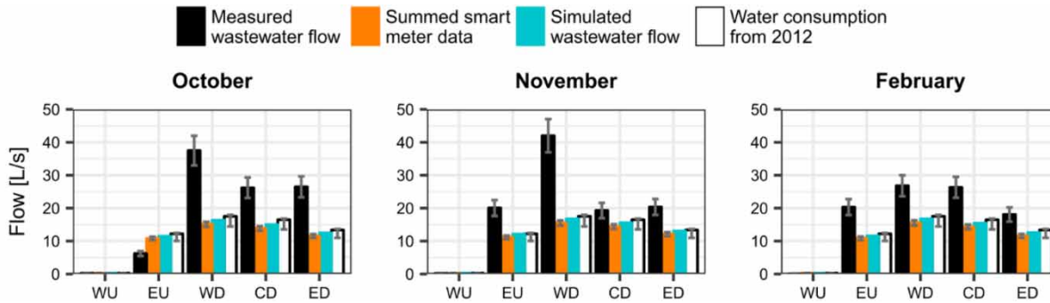
Figure 4 | Average observed flow to the WWTP ( \bar{Q}_{obs} ), summed smart meter data ( \bar{Q}_{SM} ) and simulated flow ( \bar{Q}_{sim} ) (Equation (2)) over the three time periods for each sub-catchment compared with the average consumption measured independently in 2012 ( \bar{Q}_{consumption,2012} ). The error bars of \bar{Q}_{obs} and \bar{Q}_{SM} indicate the declared uncertainties (Table 1) and are calculated as \bar{Q} \pm \bar{Q} \cdot \text{uncertainty} . The error bars of \bar{Q}_{consumption,2012} likewise indicate the declared uncertainty (Table 1) as well as the seasonal variation ( \pm 10\% ) and has furthermore been shifted downwards to reflect a decrease in water consumption between 2012 and 2018 of 8%.
