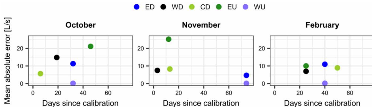
Figure 7 | Days since last calibration of in-sewer sensors compared with the difference between observed flow ( Q_{\text{obs}} ) and simulated flow ( Q_{\text{sim}} ) calculated as the mean absolute error for the three time periods.
