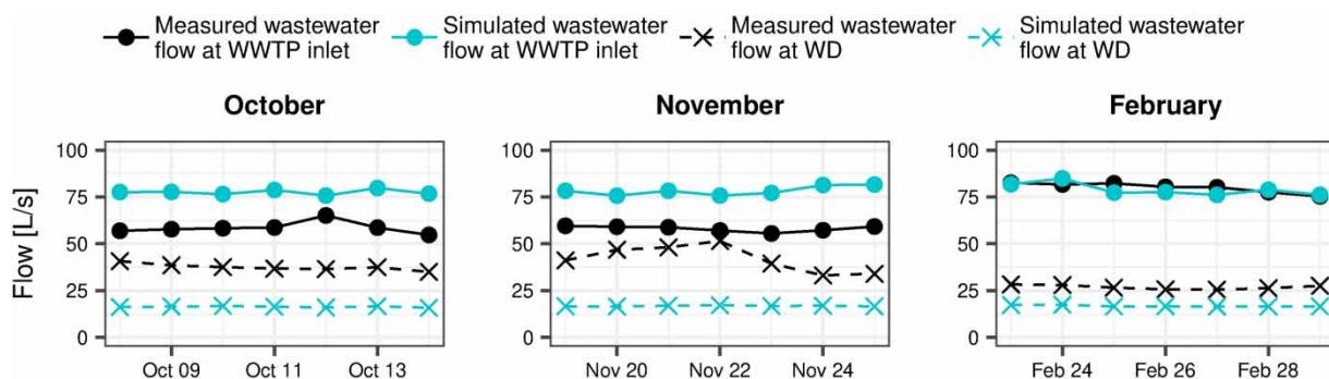
Figure 3 | Observed and simulated flows at the WWTP inlet ( Q_{\text{obs,WWTP}} vs. Q_{\text{sim,WWTP}} ) and at the sensor location West Downstream (WD) ( Q_{\text{obs,WD}} vs. Q_{\text{sim,WD}} ) in the three time periods.
