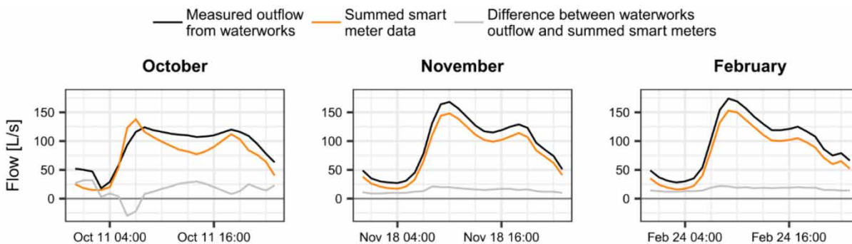
Figure 2 | Hourly outflow data from the four waterworks and water tower ( Q_{\text{obs,WW}} ) compared with summed smart meter data ( Q_{\text{SM,Elsinore}} ) for the whole of Elsinore for single days in the three time periods. Note that measured outflow data for October are incomplete.
