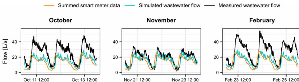
Figure 8 | Observed sewage flow ( Q_{\text{obs}} ) compared with simulated flow ( Q_{\text{sim}} ) and summed smart meter data ( Q_{\text{SM}} ) for 3 days in each of the three time periods for the 'CD' catchment.
