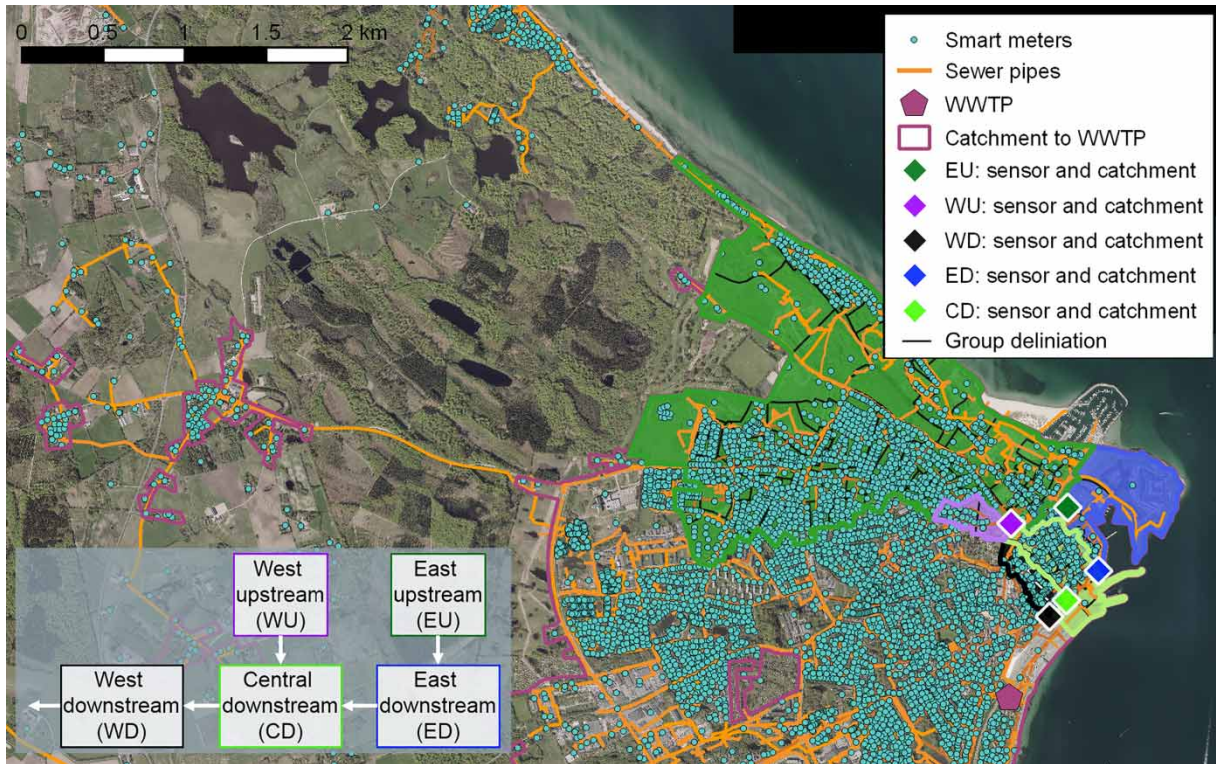
Figure 1 | Map of part of Elsinore, Denmark, showing smart meters, the sewer system, five in-sewer flow observation locations with related sub-catchments (sub-divided into 111 smaller groups for smart meter aggregation), the WWTP and the catchment discharging water to the WWTP. The flow between the sub-catchments in the sewer system is displayed in the lower left corner. EU, ED, CD, WU and WD contain 1,558, 64, 214, 45 and 134 meters, respectively. The extent of the urban drainage system and water supply system goes beyond what is shown in the figure.
