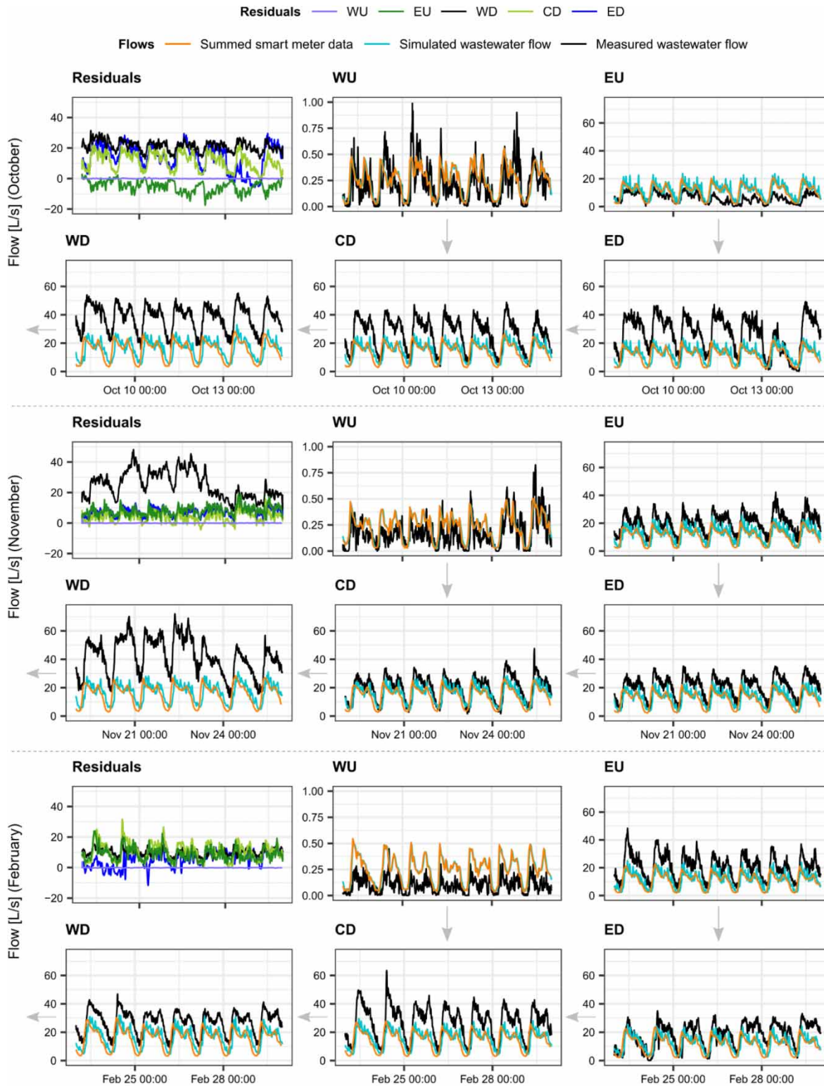
Figure 6 | Summed smart meter data ( Q_{SM} ) and simulated ( Q_{sim} ) and observed ( Q_{obs} ) sewage flows in October (top panel, Mon-Sat), November (middle panel, Mon-Sun) and February (lower panel, Sat-Fri) (Equation (1)). All data are in local time. For Q_{sim} and Q_{obs} , a 30 min moving average filter has been applied for better readability. Notice the different scales used for Residuals, WU and the four remaining plots. Due to the small flow in WU, the residuals appear constant in the Residuals plot.
