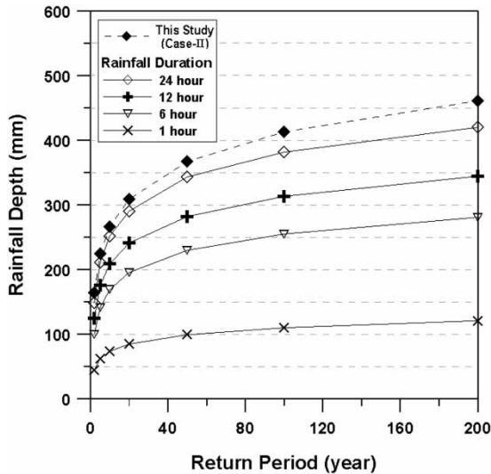
Figure 3 | Comparison results of rainfall quantiles between the conventional frequency analysis method (solid line) and this study (Case-II) with any rainfall durations (dashed line).
