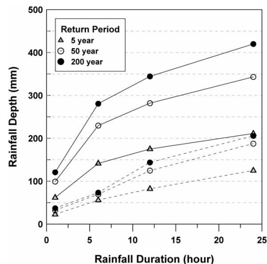
Figure 2 | Rainfall depth–duration–frequency relationships by the conventional frequency analysis method (solid line) and this study (Case-I) under the rainfall depth threshold of 10 mm/storm (dashed line).
