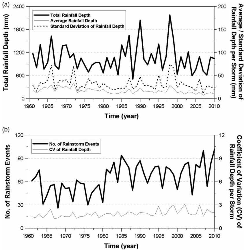
Figure 1 | Time series of annual statistics for independent rainstorm events: (a) total rainfall depth (mm), average rainfall depth per storm (mm), and standard deviation of rainfall depth per storm (mm); (b) number of storm events and coefficient of variation of rainfall depth per storm.
