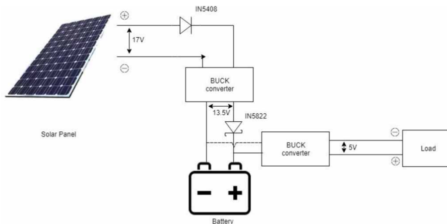
Figure 7 | Power supply.
