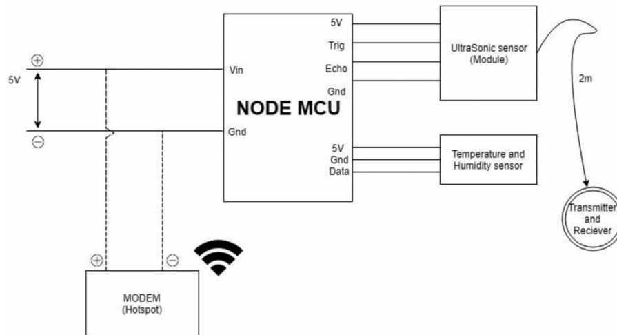
Figure 6 | Sensor network.
