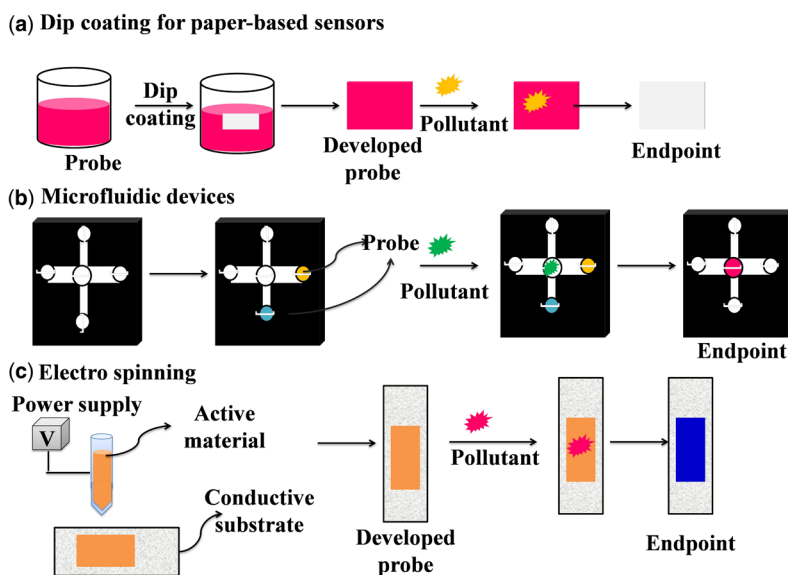
Figure 18.3 Methods for development of portable colorimetric sensors.
