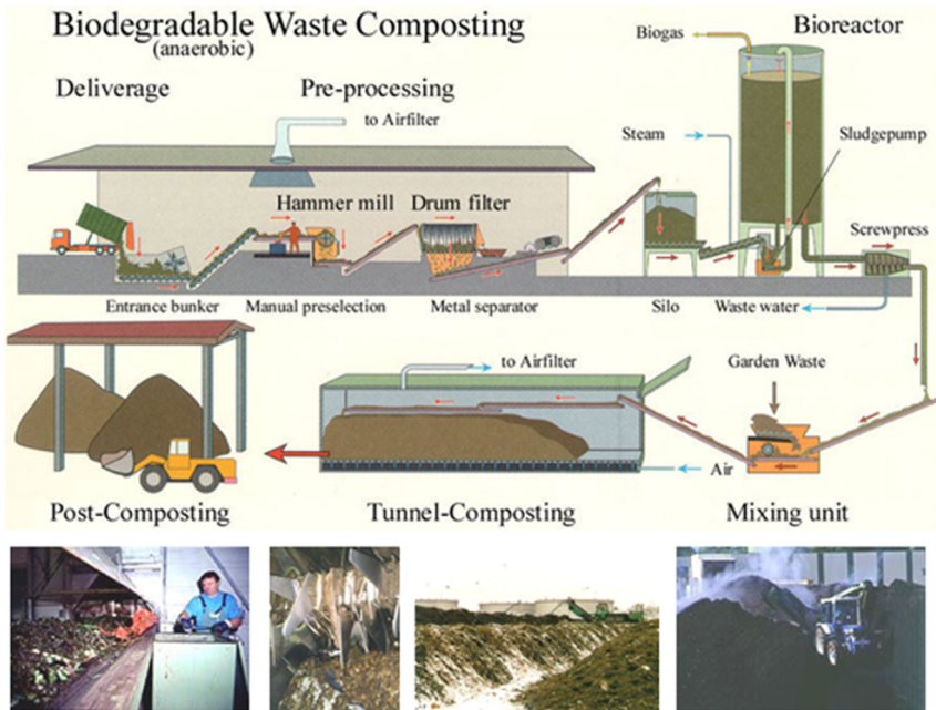
Figure 10.24 Industrial composting process (Source: Yip & Madl, 2003).
