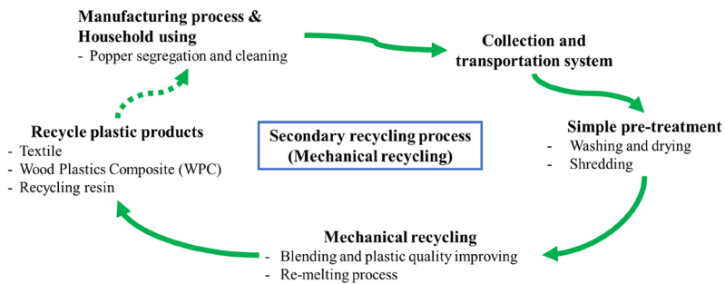
Figure 6.37 Concept of secondary recycling process.
