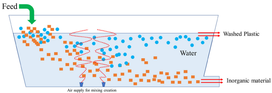
Figure 6.19 Floating washer.
