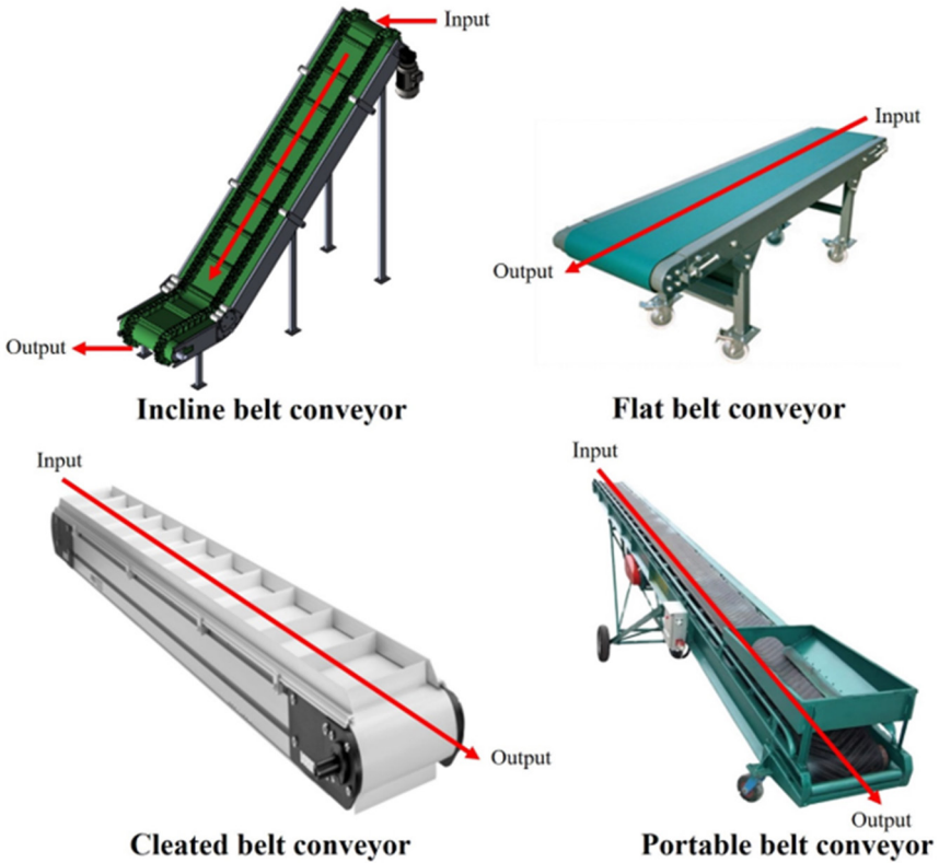
Figure 6.10 Conveyor belt used for lightweight materials (Source: modified from https://www.beidou.com/construction/belt-conveyor-types.html ).
