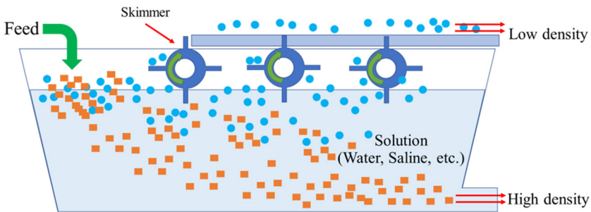
Figure 6.24 Sink-float separation.
