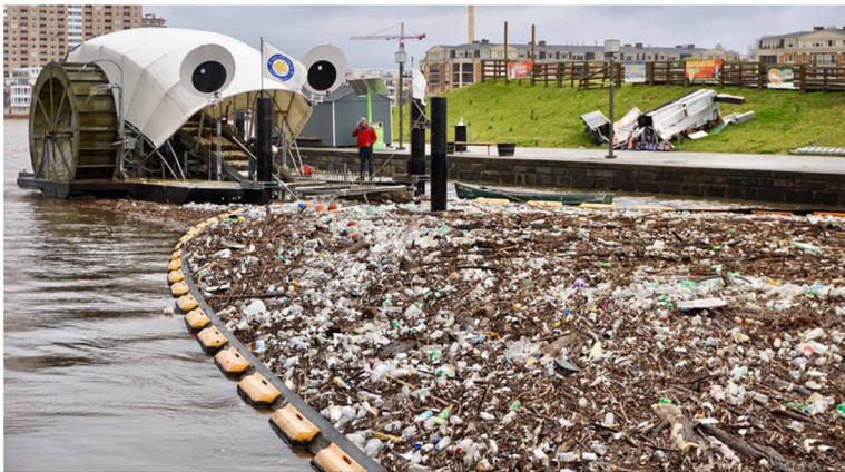
Figure 11.38 Mr. Trash Wheel (cnet.com, 2021).
